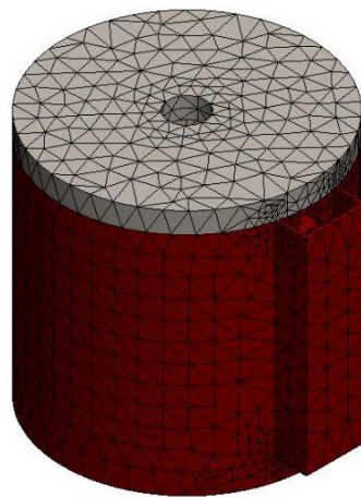
Figure 6: Meshed model for compression analysis
