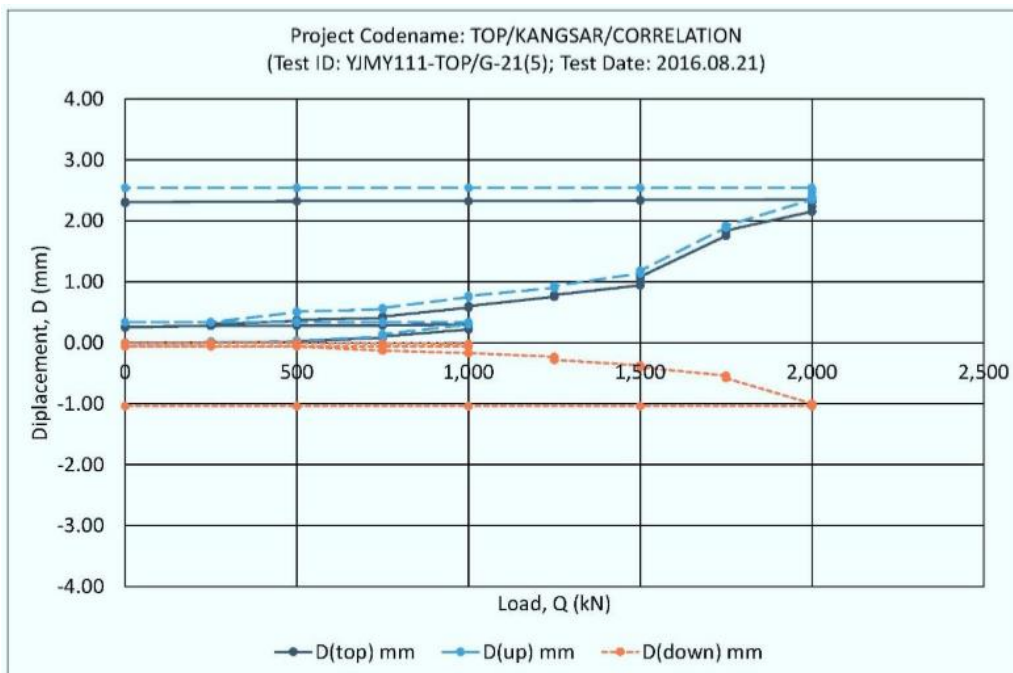
Figure 5.2: YJACK bidirectional pile test result – G-21(5)
