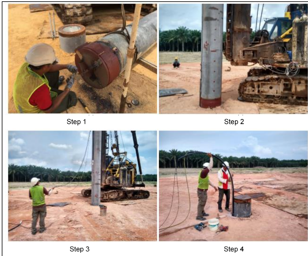
Figure 2.2: YJACK type C installation process
