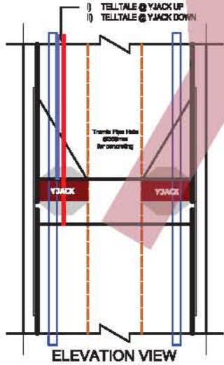
YJACK Technology (Static Maintained Load Test Method)
